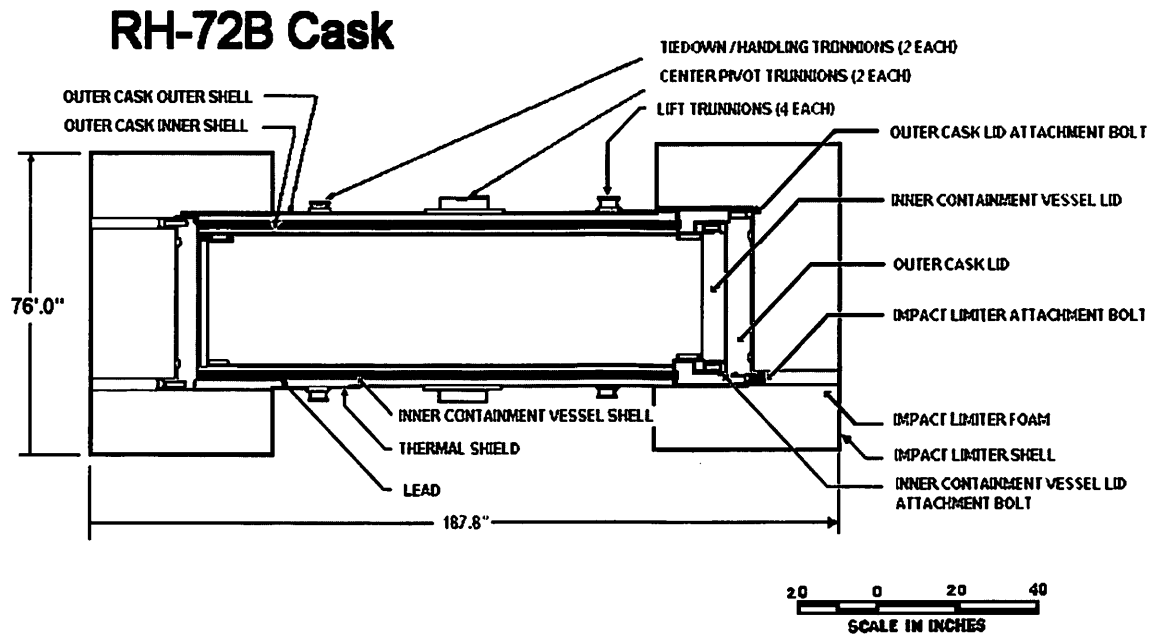
Figure 3 Cutaway of RH-72B Cask
